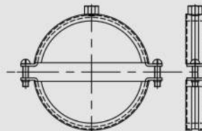
TUBE HANGER
